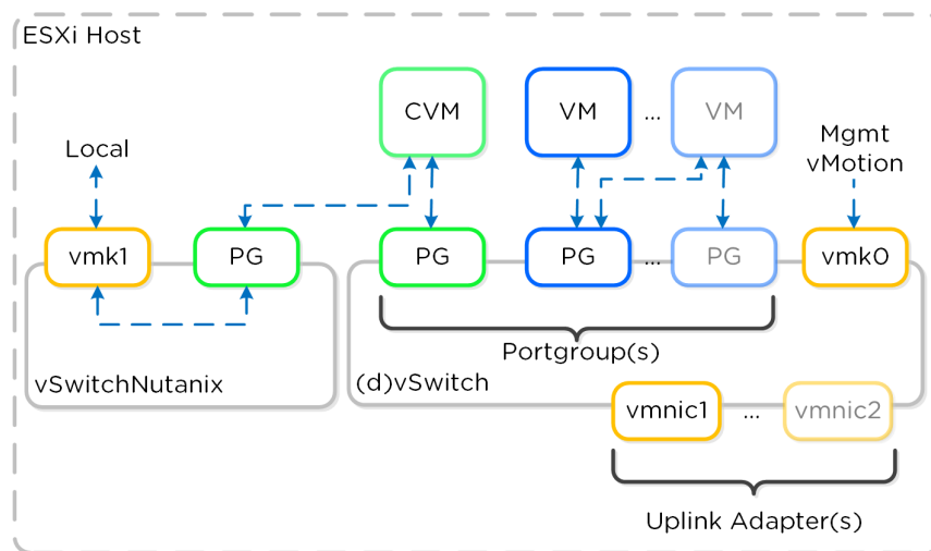
ESXi vSwitch Network Overview
